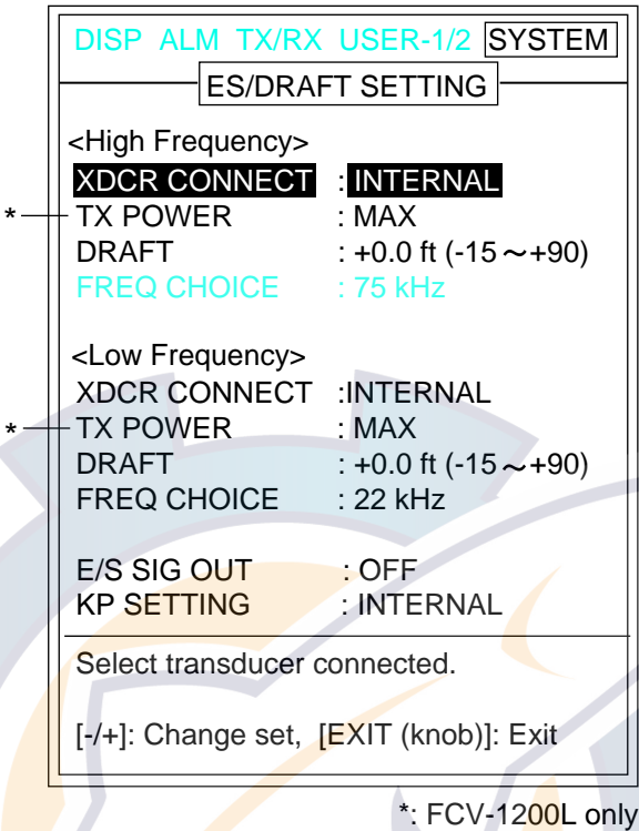
ES/DRAFT SETTING menu
