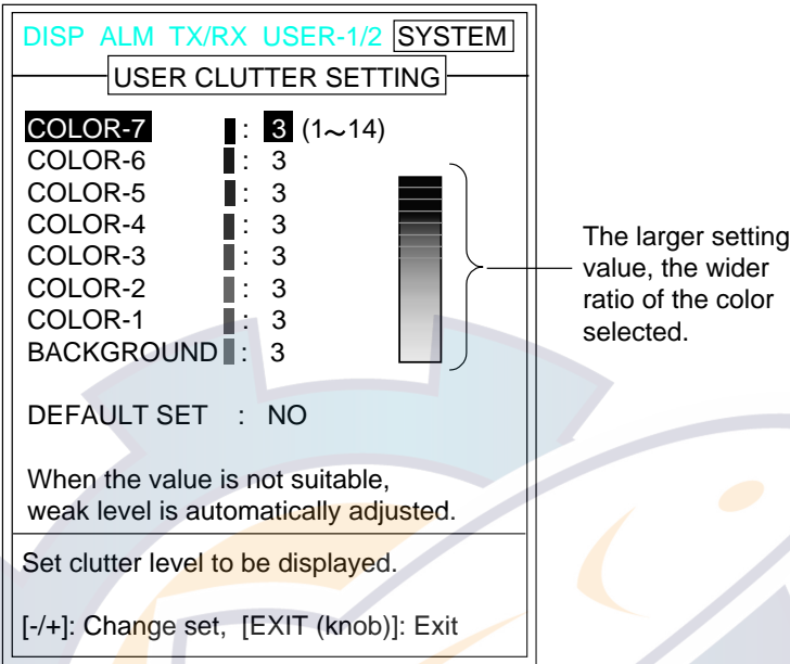
USER CLUTTER SETTING menu
