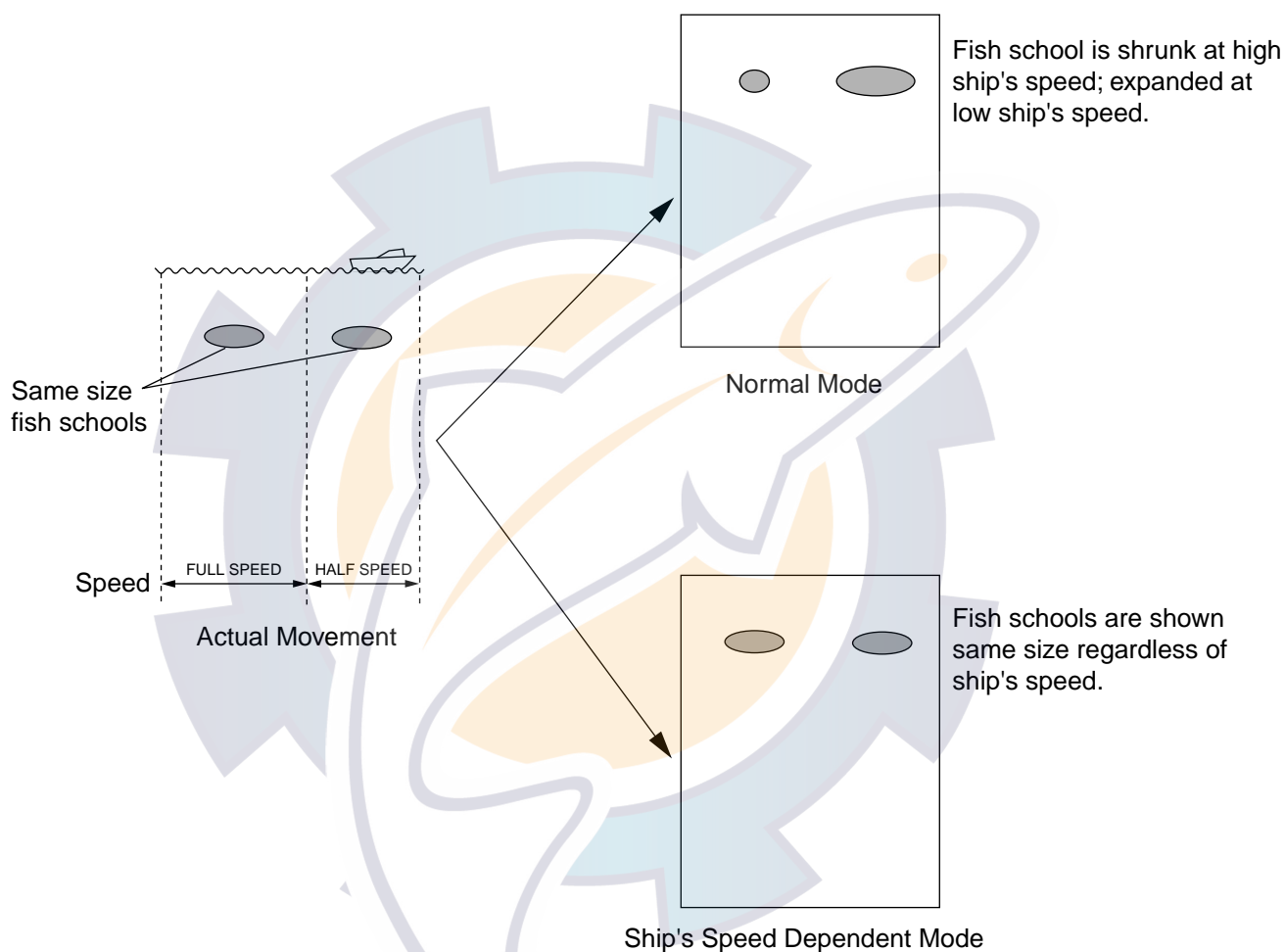
How the ship's speed dependent mode works
